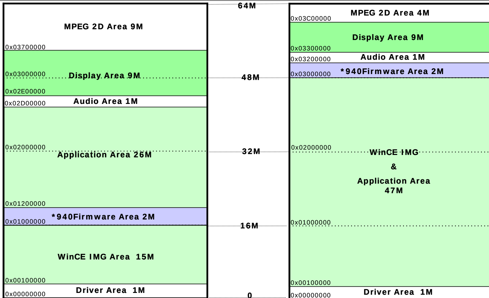
64M Limit Spec Memory Map
