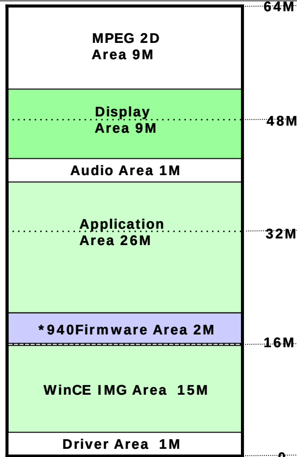
64M Full Spec Memory Map
