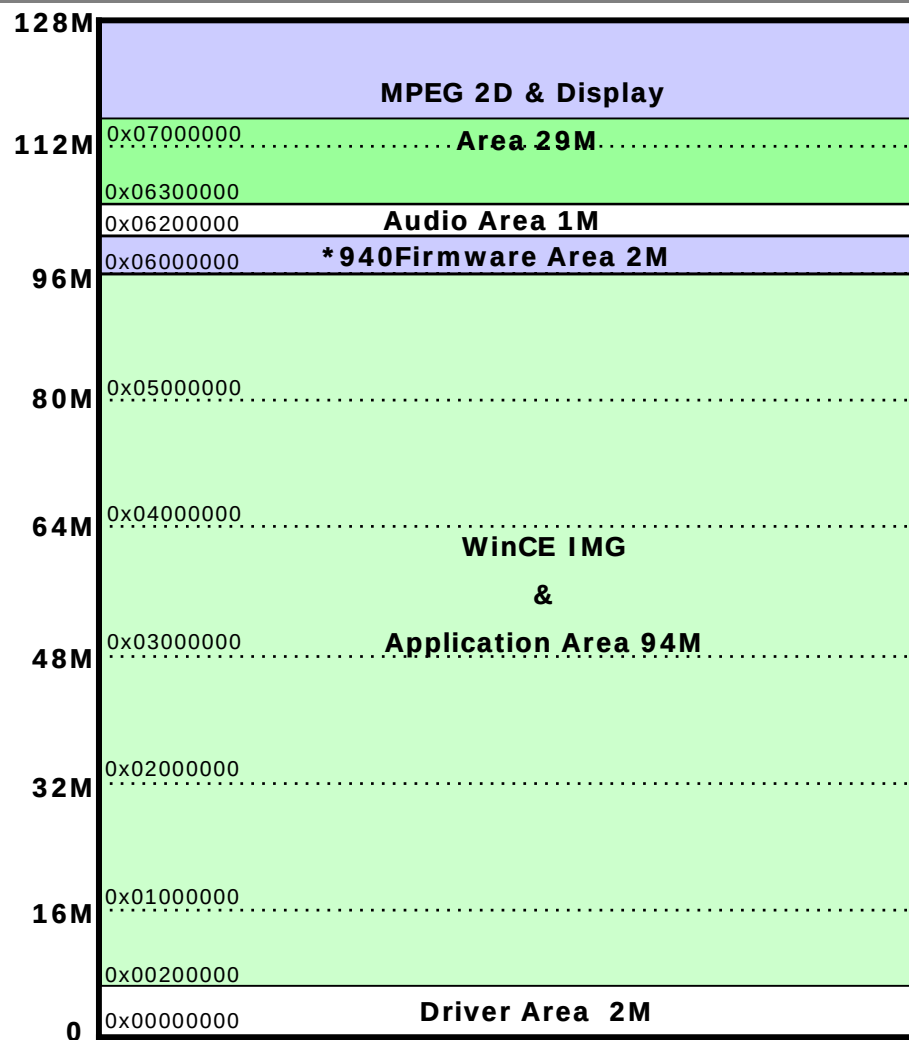
128M Full Spec Memory Map
