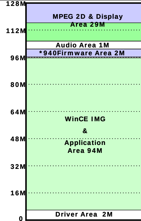
128M Full Spec Memory Map
